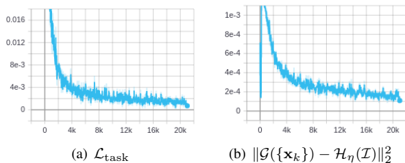
Figure 7. Evolution of the loss and heatmap during training on MNIST hard . (a) the task (classification) loss \mathcal{L}_{\text{task}} and (b) the heatmap related loss \|\mathcal{G}(\{\mathbf{x}_k\}) - \mathcal{H}_\eta(\mathcal{I})\|_2^2 for each iteration.
