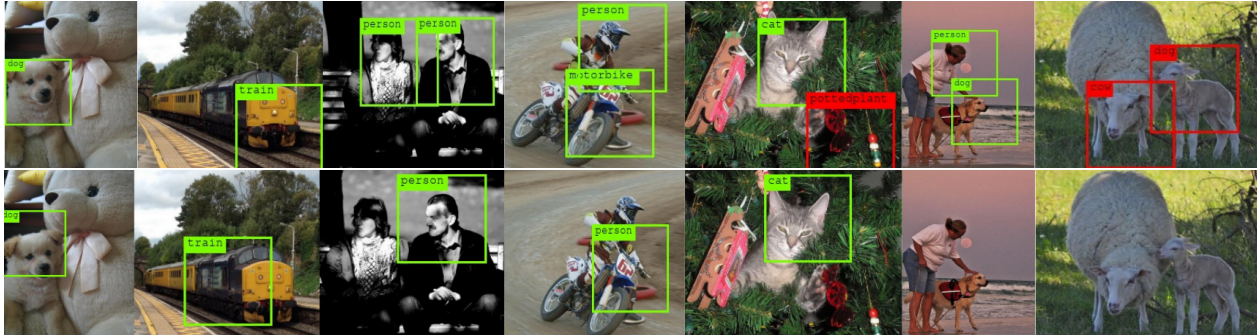
Figure 6. Qualitative results on PASCAL+COCO dataset. (Top row) we show detection results when using MIST and (bottom row) when using Xie20 [57]. Correctly localized and classified ones are shown in green, and wrong ones in red.
