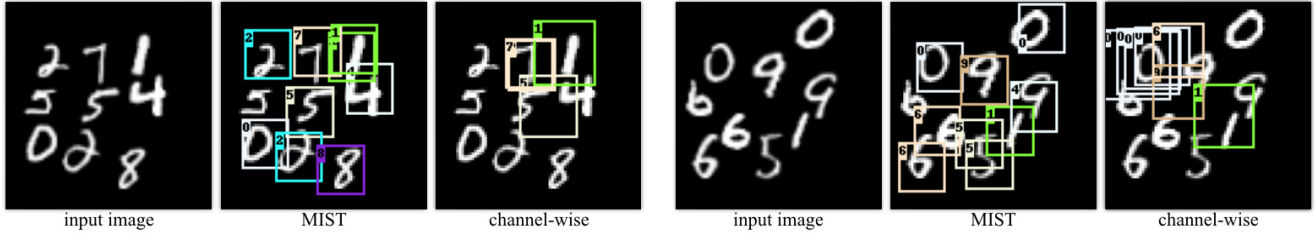
Figure 5. Two qualitative examples for detection and classification on our MNIST-hard dataset.
