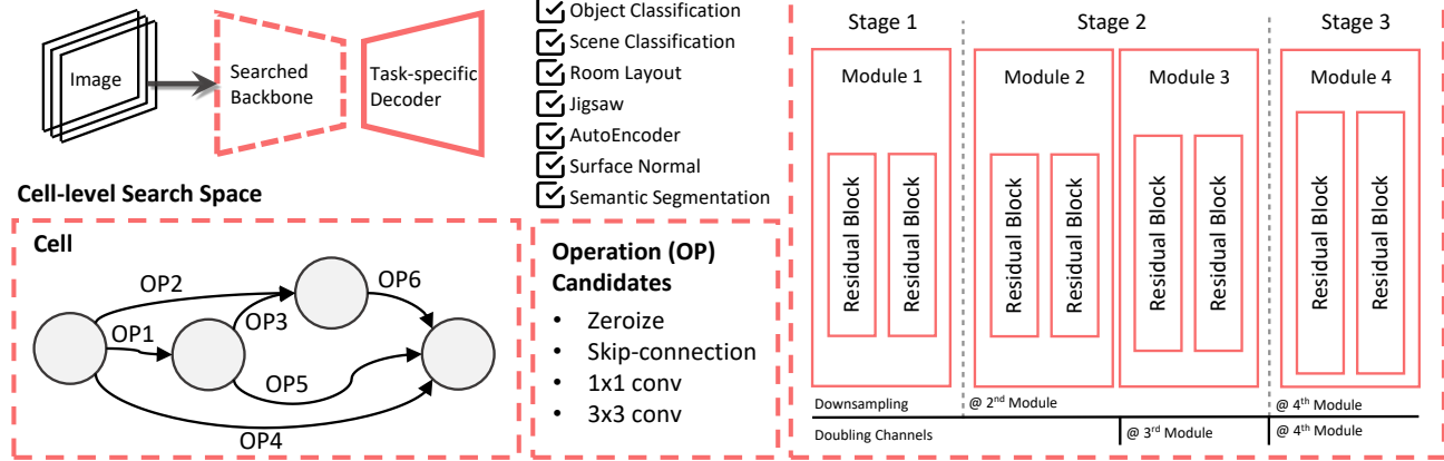
Figure 1: Our cell-level and macro-level search space in TransNAS-Bench-101. We design a cell-level search space that treats each cell as a DAG and a macro-level search space that allows flexible macro skeleton network design.
