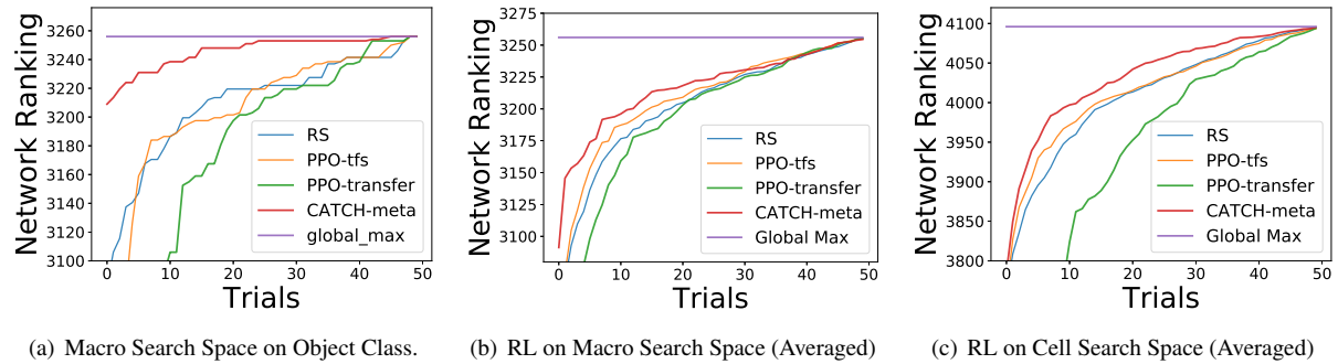
Figure 7: Comparison of PPO and CATCH. CATCH largely improves PPO-transfer’s performance, and it works exceedingly well on object classification. Similar to REA, We ran each algorithm in 7(a) for 50 trials and each trial to search 50 networks. 7(a) shows sorted search results on object classification. Each curve in 7(b) and 7(c) averages search results across all tasks.
