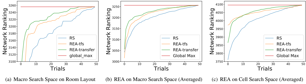
Figure 6: Comparisons of the transfer and train-from-scratch (tfs) results of REA. REA-transfer has slight but stable improvements across all tasks. We ran each algorithm in 6(a) for 50 trials and each trial to search 50 networks. We pick the model with the highest validation score in history as the search result of a trial. 6(a) shows sorted search results of on Room Layout. Each curve in 6(b) and 6(c) averages the search results across all tasks.
