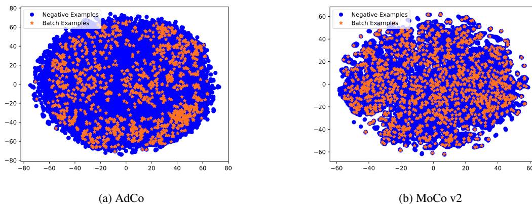
Figure 2: t-SNE visualization of negative representations obtained by the AdCo and the MoCo in the 2D representation plane, alongside positive examples from the most recent six minibatches after 200 epochs of pretraining on the ImageNet. The figure shows that the AdCo has fewer outliers of negative examples than the MoCo v2, and thus more closely tracks the representation of positive samples over epochs.
