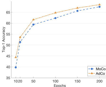
Figure 1: Top-1 accuracy of AdCo and MoCo V2 on ImageNet fine-tuned with a single fully connected layer upon the backbone ResNet-50 networks pretrained over up to 200 epochs. For a fair comparison, the AdCo maintains the same size ( K = 65, 536 ) of negative samples as in MoCo v2 so that both models are directly compared under various numbers of epochs. With an extremely small number of 10 epochs, the AdCo performs much better than the MoCo v2 by more than 5% in top-1 accuracy. As the epoch increases, the AdCo usually achieves the performance comparable to that of the MoCo v2 with about 30 ~ 50 fewer epochs. This shows the AdCo is more efficient in constructing a more critical collection of negative adversaries to improve network pretraining.
