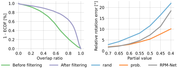
Figure 9: Improved relative overlap ratio after filtering the points with the inferred overlap scores on 8862 ModelNet partial scans ( left ). Owing to the improved overlap ratio, PREDATOR is robust to the changes of partial value p_v , while the performance of RPM-Net drops rapidly ( right ). rand and prob. denote the random and prob. (om) biased sampling of 450 interest points, respectively.
