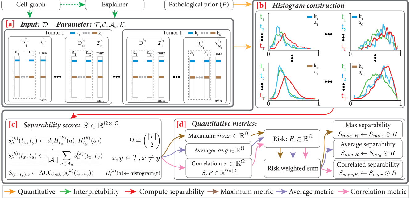
Figure 3. Overview of proposed quantitative assessment. (a) presents input dataset \mathcal{D} , and parameters concepts \mathcal{C} , measurable attributes \mathcal{A}_c , classes \mathcal{T} , and importance thresholds \mathcal{K} . For simplicity |\mathcal{A}_c| = 1, \forall c \in \mathcal{C} in this figure. (b) shows histogram probability densities for \forall a \in \mathcal{A}_c, \forall k \in \mathcal{K}, \forall t \in \mathcal{T} . (c) displays the algorithm for computing class separability score S . (d) presents the algorithm for computing the proposed class separability-based risk-weighted quantitative metrics.
