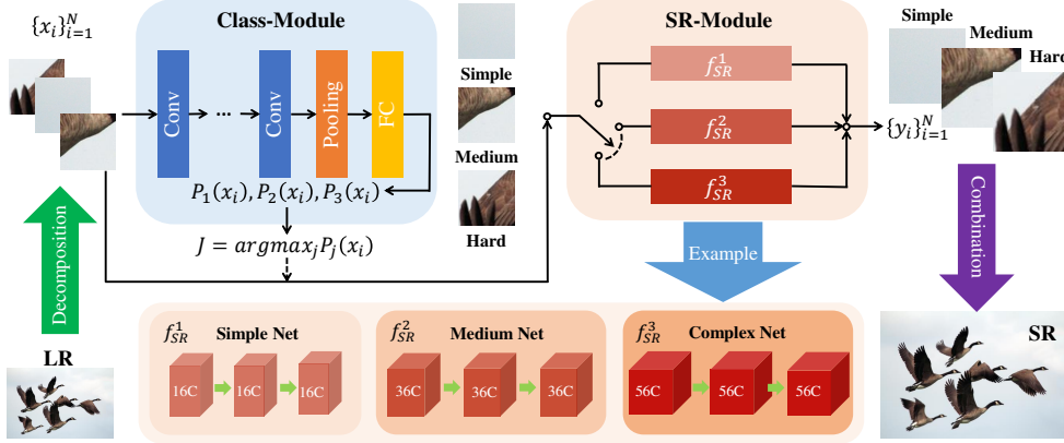
Figure 4. The overview of the proposed ClassSR, when the number of classes M = 3 . Class-Module: aims to generate the probability vector, SR-Module: aims to deal with the corresponding sub-images.
