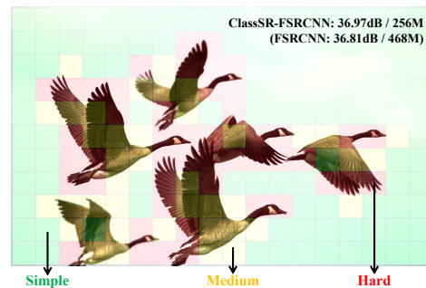
Figure 1. The SR result (x4) of ClassSR-FSRCNN. The Class-Module classifies the image “0896” (DIV2K) into 56% simple, 20% medium and 24% hard sub-images. Compared with FSRCNN, ClassSR-FSRCNN uses only 55% FLOPs to achieve the same performance.
