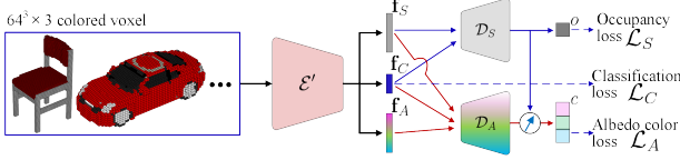
Figure 5. Colored 3D voxel encoder \mathcal{E}' and decoders pre-training.
