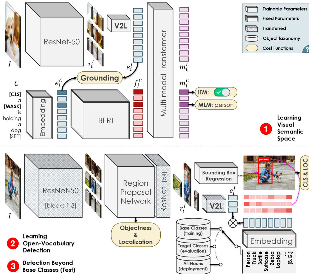
Figure 3. The architecture of our OVR-CNN during pretraining (top) and downstream training (bottom). We first train the ResNet and the V2L layer on image-caption pairs via grounding, masked language modeling (MLM) and image-text matching (ITM). Then we use the trained ResNet and V2L to initialize a Faster R-CNN in order to learn open-vocabulary object detection.
