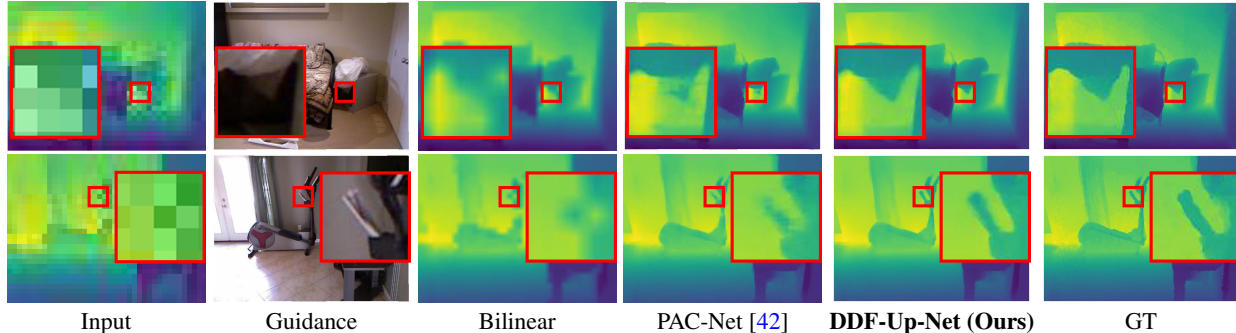
Figure 7. 16× joint depth sampling results on sample images. DDF-Up-Net recovers more depth details compared with PAC-Net [42] and other techniques.
