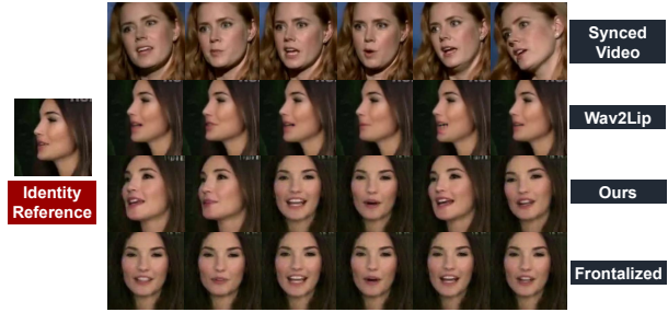
Figure 6: Results under extreme condition. We can drive faces under large poses, and even frontalize them by setting the pose code to all zeros.
