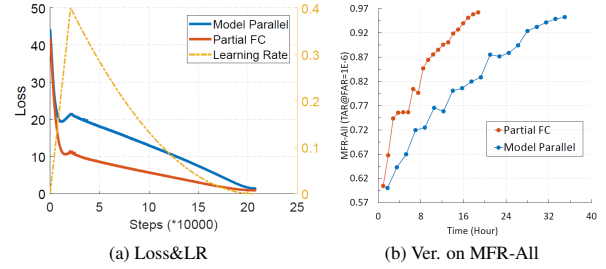
Figure 9. Training status comparisons between model parallel and PFC on WebFace42M. ResNet100 is employed here. The batch size is 128 \times 8 \times 4 .
