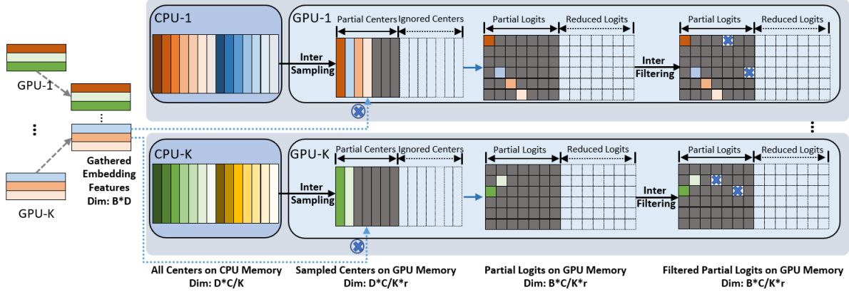
Figure 4. Distributed implementation of the proposed PFC. Face features are first gathered from each GPU. Meanwhile, partial centers are copied from each CPU to GPU. Positive class centers are picked through labels while partial negative class centers (in grey) are randomly selected to fill the buffer. After the inner product between gathered features and partial centers on each GPU, we obtain the partial logits. PFC is memory-saving and efficient because it reduces the GPU memory consumption and computation cost on the FC layer. PFC is also robust under inter-class conflict due to decreased inter-class interaction during training. On the dataset with extremely heavy inter-class conflict, abnormal inter-class high similarities can be filtered by a fixed threshold ( i.e. 0.4) in PFC to further enhance the robustness.
