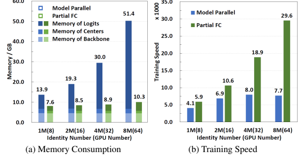
Figure 3. Memory Consumption and training speed comparisons between model parallel and PFC.
