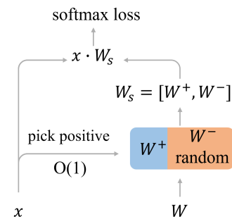
Figure 1. PFC picks the positive center by using the label and randomly selects a significantly reduced number of negative centers to calculate partial image-to-class similarities. PFC kills two birds (efficiency and robustness) with one stone (partial sampling).
