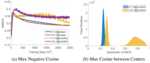
Figure 7. Inter-class statistics comparisons under different sampling ratios on the WebFace12M and WebFace12M-Conflict datasets.
