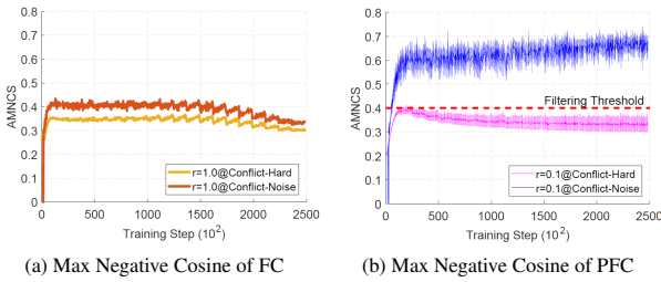
Figure 8. Hard negative and conflicted negative classes analysis under different sampling ratios on the WebFace12M-Conflict datasets.
