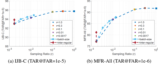
Figure 6. Verification accuracy on IJB-C and MFR-All under different sampling ratios.
