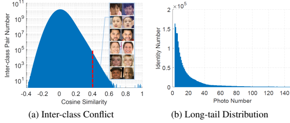
Figure 2. Inter-class conflict and long-tail distribution of WebFace42M [50].
