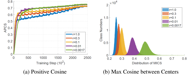
Figure 5. Intra-class compactness and inter-class discrepancy comparisons under different sampling ratios on the WebFace12M dataset.
