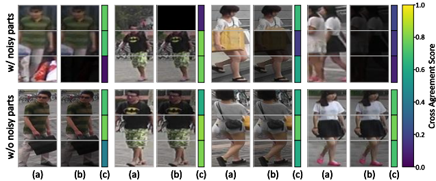
Figure 4. Visualization of cross agreement scores. (a) Original images. (b) Masked images created by multiplying the image intensity with the corresponding cross agreement score. (c) The color jet bar of the cross agreement score, where the color of each region indicates the average score over the entire training epochs.
