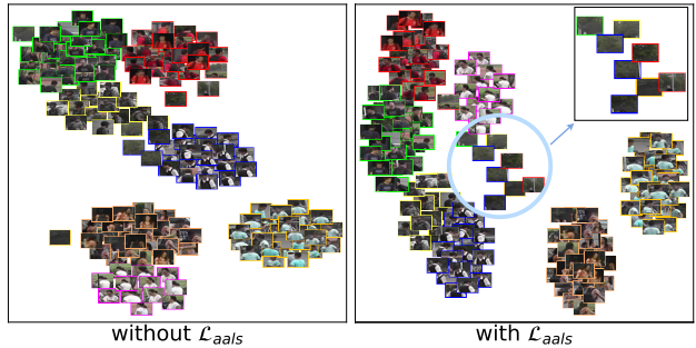
Figure 5. The t-SNE [46] visualization of the topmost part feature space of our PPLR without and with AALS. Without AALS, the embeddings overfit to ID labels and consider less the local context of each part. With AALS, it shows reliable embedding results that are well-distributed while considering the local context. The circled region shows that the features with less discriminative parts are embedded together even though their ID labels are different.
