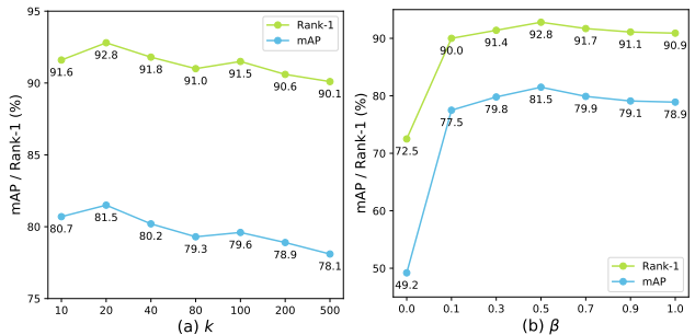
Figure 3. Parameter analysis of k and \beta on Market-1501.
