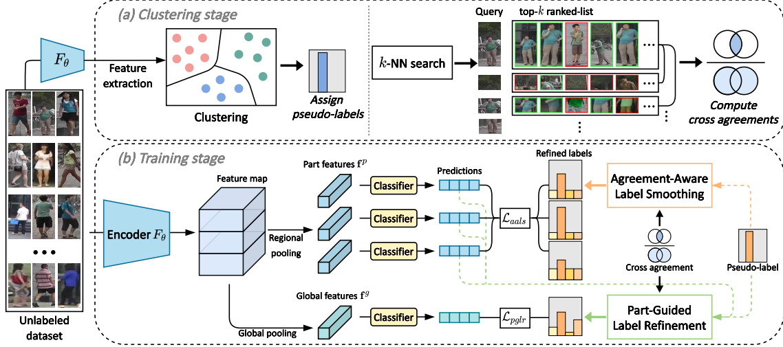
Figure 1. The illustration of PPLR. Our method alternates the clustering stage and the training stage. (a) In the clustering stage, we assign pseudo-labels by clustering the global features on the unlabeled dataset. We then perform a k -nearest neighbor search on each feature space and compute the cross agreement score based on the similarity between the top- k ranked lists of the global and part features. (b) In the training stage, we train the model with refined pseudo-labels based on the cross agreement score. We smooth the labels of part features according to the cross agreement score of each part and refine the labels of global features by aggregating the part features’ predictions.
