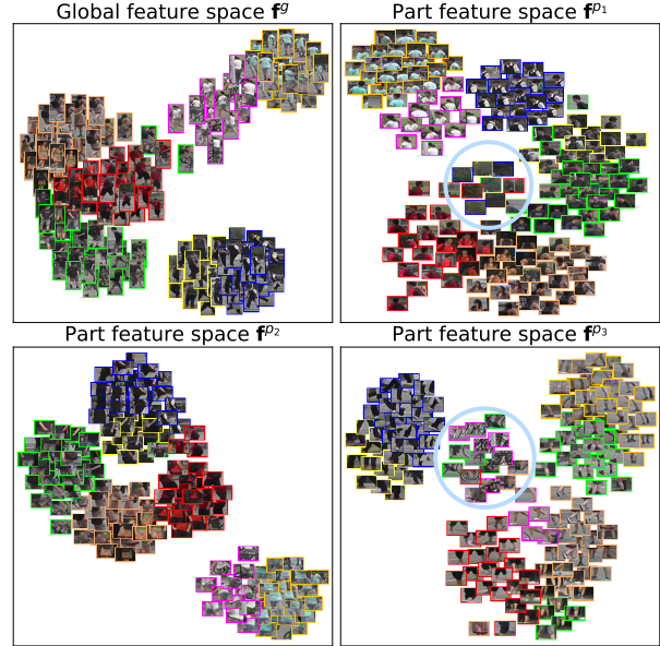
Figure 2. The t-SNE [46] visualization of each feature space on Market-1501 at an early training epoch. Different bounding box colors represent different IDs. Each feature space shows a different feature distribution with different semantic parts of a person, and some feature information can be unreliable. For instance, less discriminative parts denoted by a circle provide irrelevant information to their counterparts in other feature spaces and vice-versa. Our cross agreement score identifies such noisy information by comparing the k -nearest neighbors between feature spaces.
