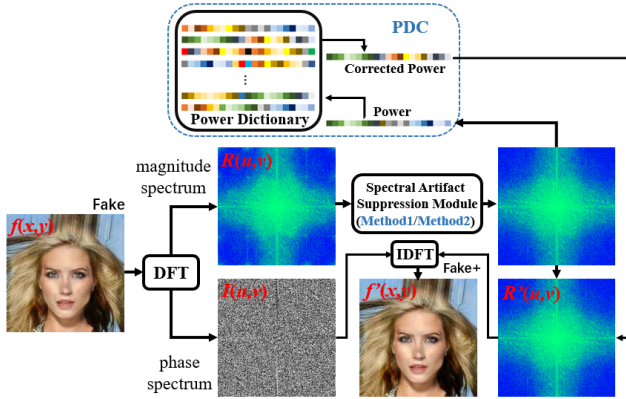
Figure 2. Our pipeline to enhance GAN-generated image to evade popular fake image detectors.
