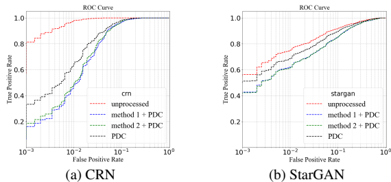
Figure 6. ROC performance curves using detector W when proposed methods are evaluated on CRN and StarGAN images.
