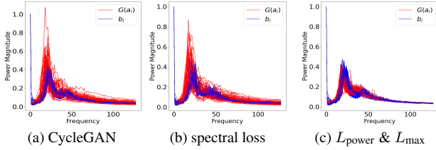
Figure 3. The comparative spectral power distributions of different optimization constraints. The blue curves illustrate the power distributions of samples b_i in domain B, the red curves illustrate power distributions of spectra which are mapped from samples a_i in domain A using function G .
