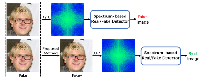
Figure 1. Detectors based on the artifacts in frequency spectrum of GAN-generated images show good performance in recent works. However, these detectors can be compromised when the GAN-generated images are further subjected to our proposed methods.
