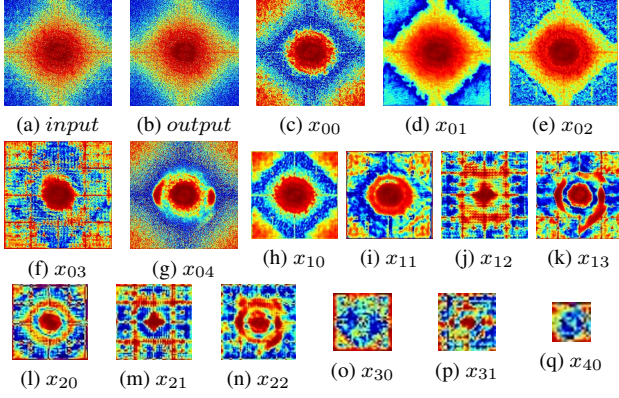
Figure 4. Intermediate features during forward propagation .
