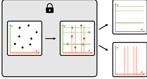
Figure 2. Disjoint map creation: To generate multiple, disjoint maps we split the original point cloud and project each point to its assigned coordinate axis. Afterwards, we distribute only the computed plane offsets along the coordinate axes to the servers. The original point map could reveal private information, so the map generation needs to be performed in a trusted environment. We show the 2D case for simplicity, but the same process trivially generalizes to 3D.
