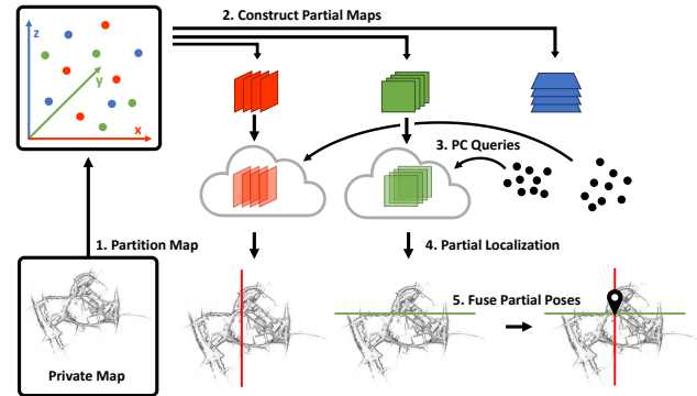
Figure 1. System architecture: We lift the original point cloud map to privacy-preserving parallel plane maps to only allow constraints in a single direction. This can be duplicated with multiple maps and localization services to accumulate different constraints locally. The clients send their localization queries to each server, which compute partial camera localization poses. Only the client can assemble the full localization result from the partial answers. Although we need three orthogonal maps for full 6 DoF pose estimation, additional constraints, such as localization in the ground plane, can reduce this requirement.
