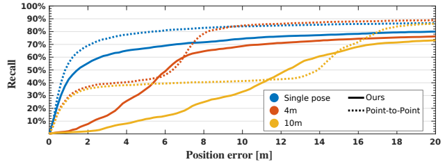
Figure 7. Disjoint query precision-recall: 2D position precision-recall plot with poses combined from two queries at the same pose, and with 4m and 10m distance between the queries using the RobotCar dataset. Relative poses between the two query locations are computed using the provided INS data. Point-to-Point alignment combines the constraints of both queries using the same relative pose estimate.
