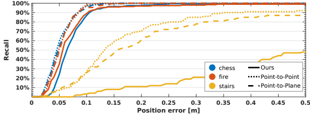
Figure 8. Depth sensor precision-recall: Position precision-recall plot for a subset of 7 scenes. For most scenes accuracy and robustness of our method is comparable with the baselines. Please refer to the supplementary material for the remaining scenes.
