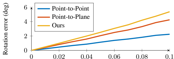
Figure 4. Noise sensitivity: The average rotation error (degrees) versus standard deviation. Note that the width of the point cloud is one.
