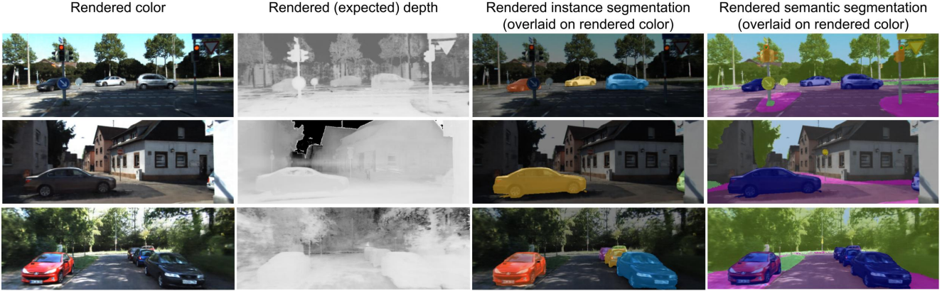
Figure 6. Images of color, depth, instance segmentation, and semantic segmentation rendered on dynamic KITTI scenes from our model trained only from RGB images.
