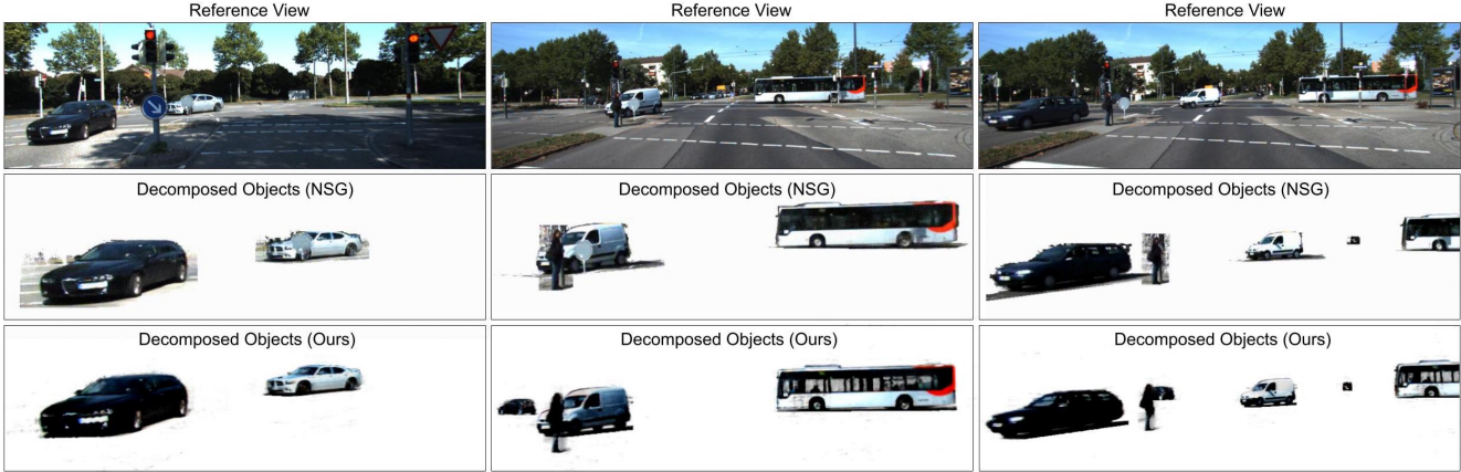
Figure 9. Scene decomposition comparison. Top row: reference views. Middle and Bottom: renderings of objects (without background stuff) of NSG [40] and PNF (ours) model respectively. Note that the traffic sign-posts in front of the cars are entangled with the rendered cars in NSG, but not in our results. Also the windows of the bus are correctly reconstructed as translucent by our model.
