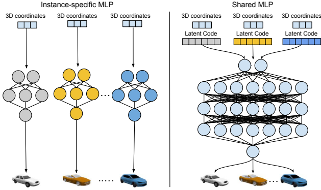
Figure 3. Our framework uses instance-specific fully weight encoded functions to represent each object (left), in comparison to a traditional approach of using one shared MLP with instance-specific latent codes (right). Instance-specific MLPs can be smaller, since they just need to have enough capacity to express a single object instance, as compared to a shared MLP. On scenes with multiple objects our approach can be significantly faster.
