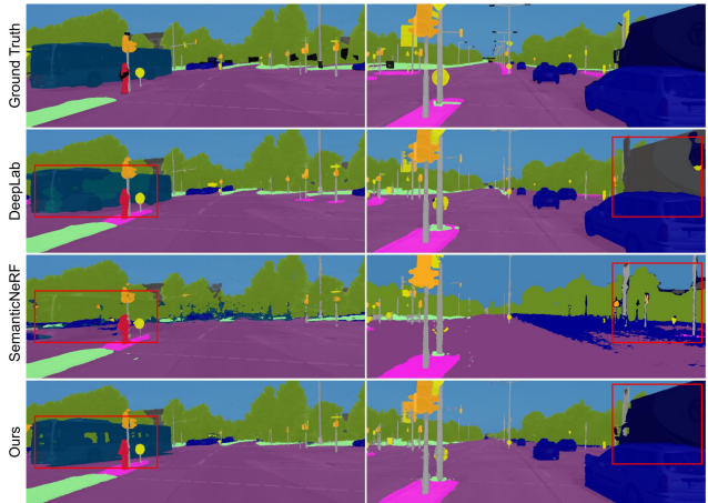
Figure 8. Comparison of semantic segmentation output from Panoptic-DeepLab [6] on ground-truth RGB image, SemanticNeRF [66], and the semantic segmentation rendered from our model from the same view. Segmentation produced by our model is significantly better as highlighted by the red boxes in the figure.
