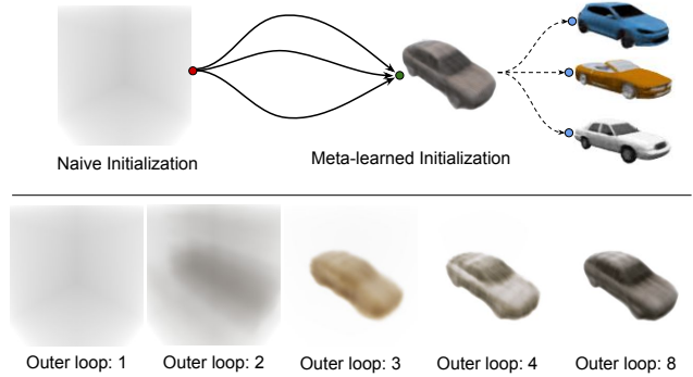
Figure 5. Category specific learned initialization with federated averaging. Upper: Rather than random initialization of MLP weights, we use meta-learning implemented using FedAvg [23,32] to find a good category specific initialization. This allows improves generalization and convergence behavior. Lower: We visualize the learned initialization model for the car class with increasing outer loops of the federated averaging algorithm.
