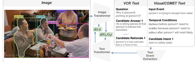
(b) Architecture of VCR and VisualCOMET. We rank ⟨question, answer⟩ and ⟨input event, temporal condition, intent⟩ respectively given the image. We calculate both the image-text level alignment and the event graph alignment.
