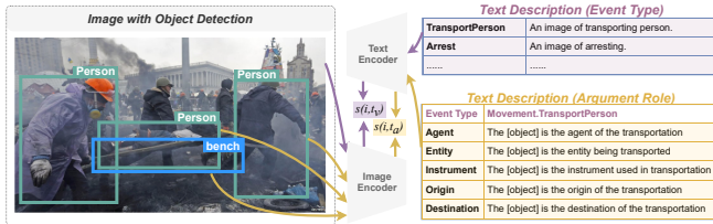
(a) Architecture of event extraction ( M^2E^2 and GSR). Event typing (in purple) ranks event type descriptions given the image, and argument extraction (in yellow) rank argument descriptions given the bounding box.
