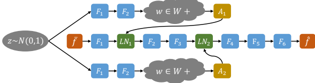
Figure 5. The architecture of our shape-IMLE generator. Inspired by StyleGAN [37], we map random noise z to latent space W+ [1] to control the generator through adaptive Layer Normalization [5] ( A_1 and A_2 ) at the first and third fully-connected layers.
