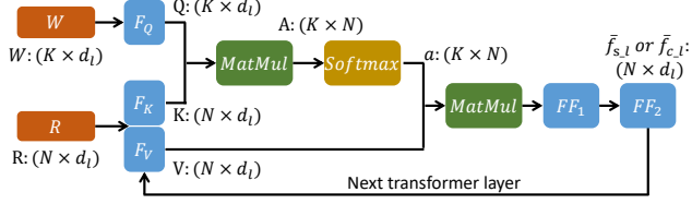
Figure 3. The Word-Level Spatial Transformer architecture. F_Q , F_K , and F_V are fully-connected layers, whereas FF_1 and FF_2 are feed-forward networks. The Layer Normalization [5] is omitted.
