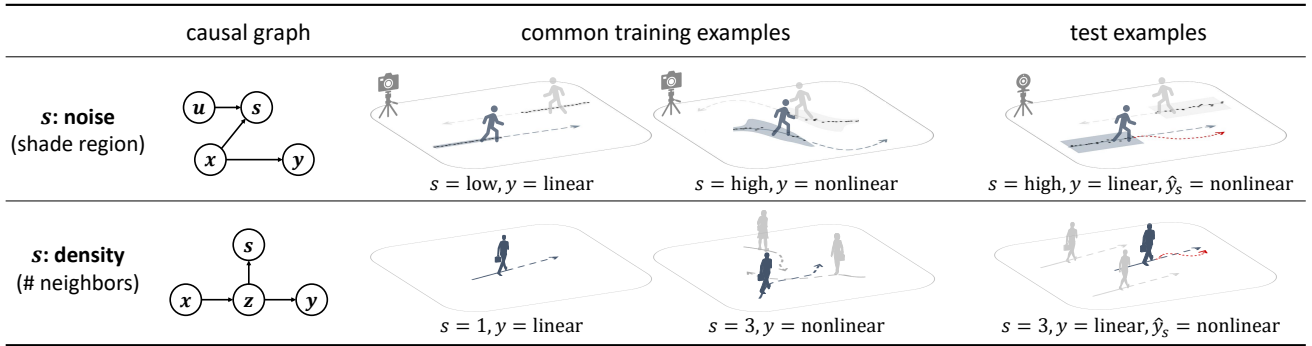
Figure 3. Illustration of spurious correlations in motion forecasting. The curvature of the target trajectory \mathbf{y} is often correlated with spurious features \mathbf{s} , such as observation noises and agent densities. Yet, such correlations are not robust. For instance, the noise level may correlate with \mathbf{y} in different ways between training and test, due to the change of exogenous variables \mathbf{u} , e.g. , sensing devices. Likewise, the agent density and \mathbf{y} are not causally related, but confounded by invariant features \mathbf{z} , e.g. , neighboring environment. In the two illustrated cases, the test example is much closer to the left training example than to the right one in essence. However, models built upon the spurious correlations in the training examples may output erroneous predictions \hat{y}_s even on simple test examples.
