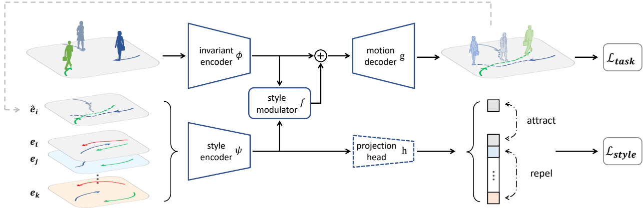
Figure 4. Our modular forecasting model contains two separate encoders for universal laws and style confounders, respectively. The model is built in three steps: (i) learn an invariant predictor based on the first encoder \phi , with the goal to be equally optimal in all training environments (§3.2), (ii) learn an embedding space based on the second encoder \psi to capture the style relation between different scenes (§3.4), (iii) incorporate domain-specific style features into the forecasting model by training \psi , f , g and h on the main task and the auxiliary style contrastive task jointly (§3.3-§3.4).
