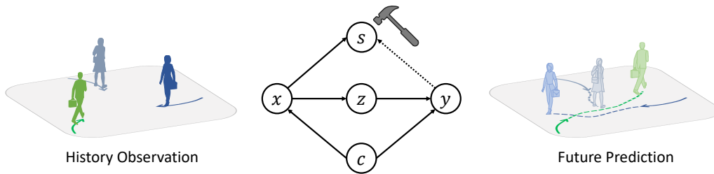
Figure 2. Our causal formalism of motion forecasting. We cast the human motion problem as a dynamic process with three groups of latent variables: domain-invariant physical laws ( z ), domain-specific style confounders ( c ), and non-causal spurious features ( s ). The spurious features are not parents of future movements ( y ) in the causal graph, e.g. , no edges or anti-causal (dotted line), and their statistical correlations may vary drastically under different conditions. This formalism motivates our design and training of forecasting models to promote the robustness and reusability of the learned motion representation.
