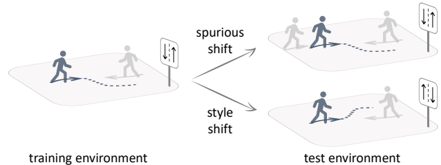
Figure 1. Illustration of motion forecasting under environment changes. We introduce a framework that enables deep motion representations to robustly generalize to non-causal shifts of spurious features, e.g., agent density, and efficiently adapt to new motion styles , e.g., from right to left-hand traffic.
