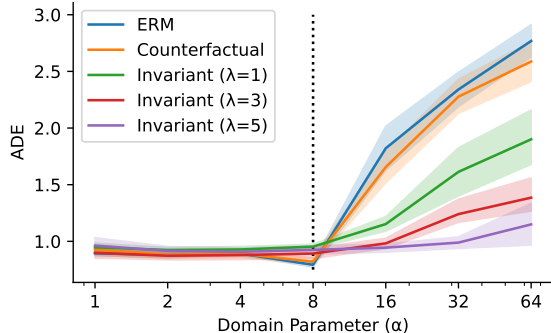
Figure 5. Comparison of different methods on the ETH-UCY dataset with controlled spurious correlations. Our invariant learning approach substantially outperforms the conventional ERM and the counterfactual approach [13] in the out-of-distribution regime \alpha \in (8, 64] , while being on par within the training domains.
