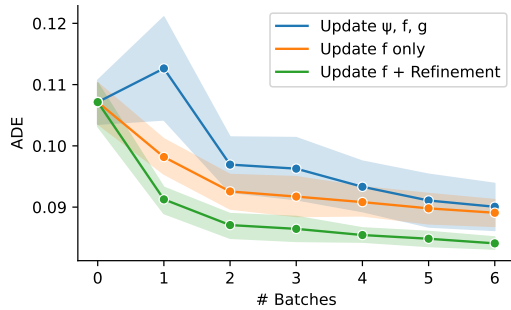
Figure 6. Quantitative results of different methods for transfer learning to a new motion style, given limited batch of samples. Our modular adaptation strategy (updating the style modulator f ) yields higher sample efficiency than the conventional counterpart in the low-data regime. Moreover, refining the predicted output for 3 iterations further reduces the prediction error on the fly.
