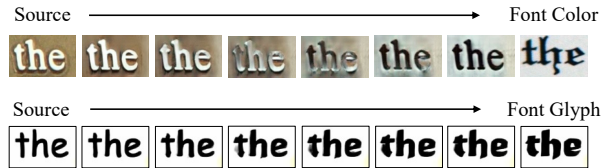
Figure 8. Font interpolation effects produced by our approach.
