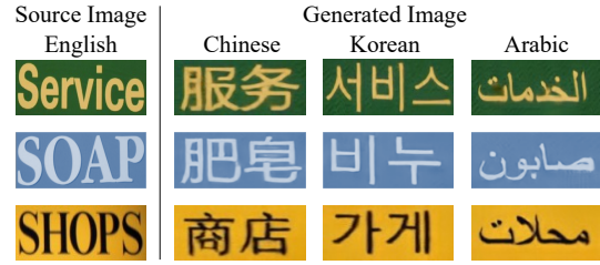
Figure 7. Cross language editing via our self-supervised approach.
