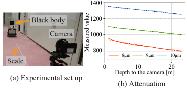
Figure 6. Experiment for measuring the extinction coefficients. (a) Experimental setup. (b) Measured values attenuated by the air. Dashed lines represent the fit curve of the Lambert-Beer law for each filter.
