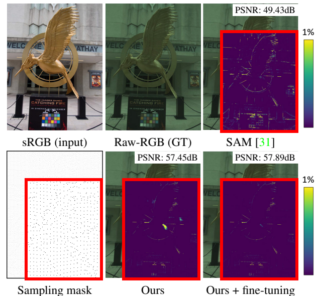
Figure 1. Overview of our paper. We address the problem of de-rendering an sRGB image to a raw-RGB image using a metadata saved along with the sRGB image. At capture time, we sample the raw-RGB values at the locations in a sampling mask, and save them as a metadata. When the raw-RGB image is needed, we reconstruct the full raw-RGB image from the sRGB image with the metadata. We propose an end-to-end deep learning framework to achieve it. With our approach, the reconstruction can be further improved by online fine-tuning.
