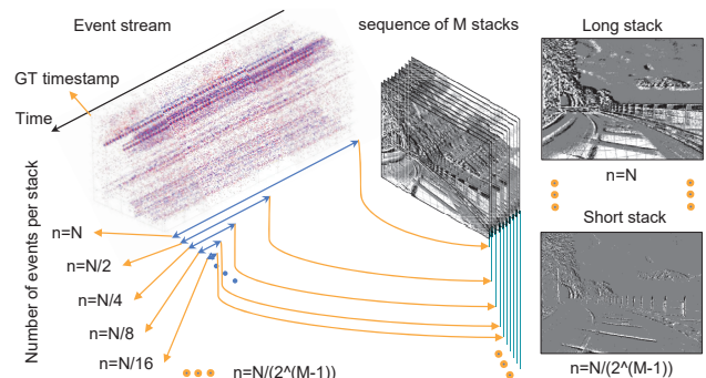
Figure 3. Event sequence creation for the ‘concentration network’. We utilize a sequence of stacks created with different numbers of events per stack. Moving backward in time from the ground-truth (GT) depth timestamp, we first stack a very large number of events that include all movements from a long time span. For the next stack, we use half of the events used in the previous slice of the event stream and use the chunk that is connected to the GT location. We continue slicing the events in half until we reach the final stack M that we choose based on the number of stacks we want to include in our attention network.
