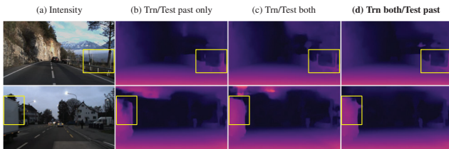
Figure 7. Qualitative results by KD from future. (both: past+future)
