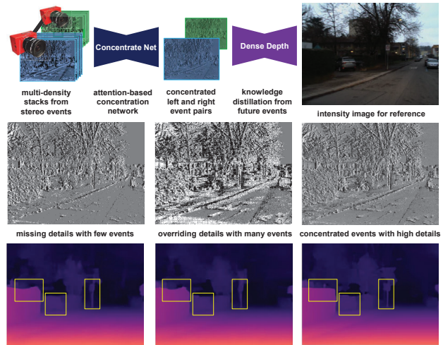
Figure 1. Overview of our stereo depth estimation from events. We predict dense depth with sharp edges by ‘concentrating’ the event representation tensors to preserve details. We further transfer the knowledge of future events by training with past and future events while keeping our system causal at inference.
