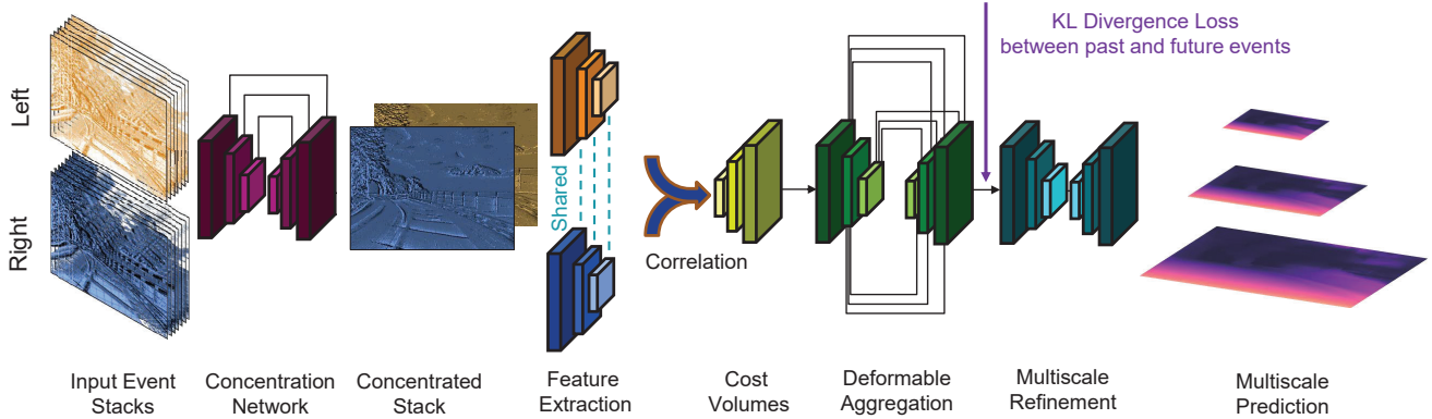
Figure 4. Architecture overview. We create a series of multi-density event stacks (Sec. 4.2) and use the concentration network (Sec. 5.1) to create the detailed event-based tensor called concentrated stack. We use the multiscale encoder to extract features (with shared weights) and correlate them to create cost volumes (Sec. 5.2). By ‘deformable aggregation’ and ‘multiscale refinement’ of the prediction we create our output dense depth estimation. Utilizing past and future events at training (Sec. 5.3) we can distill the knowledge from future events through the KL-divergence loss and reach higher quality depth estimations. The learning objectives are described in Sec. 5.4.
