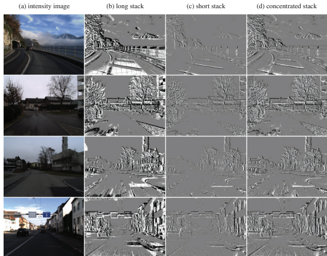
Figure 2. Shortcomings of conventional event stacking method by a number of stacks (SBN). Representing the event stream by a predefined number of events or time intervals either overwrites previous events when the number of events is large, ((b) long stack) or omits scene details when the number of events is small ((c) short stack). (d) Our concentration network produces meaningful stacks (c) without overriding or missing events. The intensity image (a) is presented for reference.
