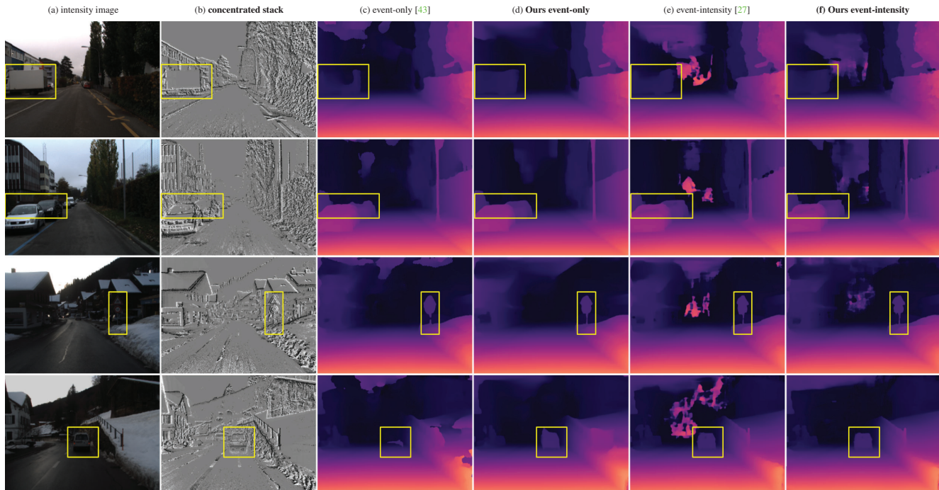
Figure 5. Qualitative comparison on dense depth estimation. We present our dense depth estimations using event-only (d) and events fused with intensity images (f) together with the (a) intensity image and (b) concentrated event stack for reference. We compare them to the (c) event-only [43] and (e) event-intensity [27] methods respectively. In the highlighted regions by yellow boxes, our method constructs fine details much better, e.g. , better clarity in cars (first, second, and fourth rows) and details of road sign with a post (third row), compared to its prior arts in both event-only and event-intensity modalities. Best viewed with the highlighted regions for detailed comparison.
