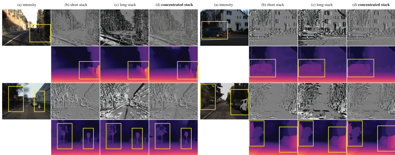
Figure 6. Effect of the number of events on depth quality. (a) intensity image, together with the depth predictions using a (b) short stack, (c) long stack, and also the (d) concentrated stack. The concentrated stack creates crisp clear boundaries and covers the scene details much better than using a fixed number of events in a stack, i.e. , short or long stacks.
