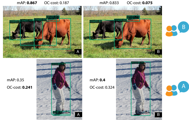
Figure 5. Examples of annotators' votes. Annotators compare two detection results and vote which one looks better. For each detection results, mAP for single image and OC-cost are displayed. OC-cost shows better agreement with human preference.
