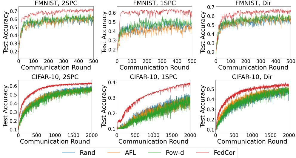
Figure 4. Test accuracy on FMNIST and CIFAR-10 under three heterogeneous settings (2SPC, 1SPC and Dir). All experiments in one figure share the same hyperparameters except for the client selection strategy.
