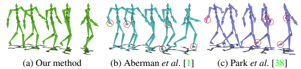
Figure 5. Style transfer results of the first ten frames. Task: Neutral walk into proud style. Noticeable artifacts of awkward joint rotations are circled in red.
