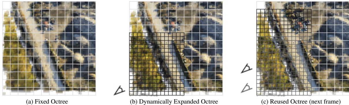
Figure 4. Mega-NeRF-Dynamic . Current renderers (such as Plenotree [45]) cache precomputed model outputs into a fixed octree, limiting the resolution of rendered images (a). Mega-NeRF-Dynamic dynamically expands the octree based on the current position of the fly-through (b). Because of the temporal coherence of camera views, the next-frame rendering (c) can reuse of much of expanded octree.
