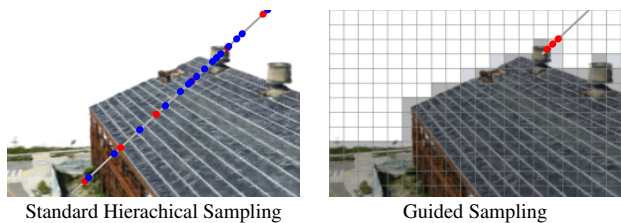
Figure 5. Guided Sampling . Standard NeRF (left) first samples coarsely at uniform intervals along the ray and subsequently performs another round of sampling guided by the coarse weights. Mega-NeRF-Dynamic (right) uses its caching structure to skip empty spaces and take a small number of samples near surfaces.
