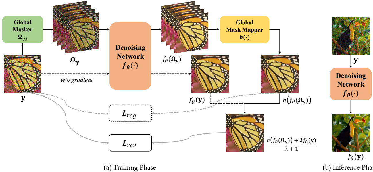
Figure 1. Overview of our proposed Blind2Unblind framework. (a) Overall training process. The global masker \Omega(\cdot) creates a masked volume by adding blind spots to a noisy image \mathbf{y} . Then, the global-aware mask mapper samples the denoised volume to obtain h(f_\theta(\Omega_{\mathbf{y}})) . Meanwhile, the denoiser f_\theta(\cdot) takes \mathbf{y} as input and produces the denoised result f_\theta(\mathbf{y}) . The re-visible loss realizes the transition from the blind to visible with the invisible term h(f_\theta(\Omega_{\mathbf{y}})) as a medium. Moreover, the regular term is used to stabilize the training phase. (b) Inference using the trained denoising model. The denoising network generates denoised images directly from noisy images \mathbf{y} without additional operation.
