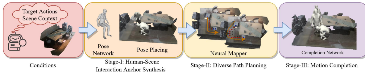
Figure 2. Overview of the framework. Our framework is composed of three stages. Given the target actions and the scene contexts, our framework first generates human-scene interaction anchors by firstly synthesizing scene-agnostic poses via the pose network and then placing the poses into the scene guided by the scene contexts and Pose Refiner. Then the framework produces diverse planning paths through the adapted A* algorithm that is amended with the novel Neural Mapper. At last, the motion completion network is leveraged to synthesize natural human motions guided by the anchors and following the planned paths.
