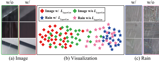
Figure 7. The effectiveness of the layer contrastive for better image and rain streaks decomposition. (a) and (c) show the decoupled rain and image patches w/ and w/o the layer contrastive. (b) visualizes the low-dimensional distributions w/ and w/o the layer contrastive.
