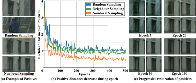
Figure 4. Effectiveness of the non-local sampling strategy. (a) Example of the randomly sampled positives with low similarity in comparison with the non-local self-similar sampled positives. (b) The Euclidean distances of positives decrease rapidly to a relative low level by non-local sampling strategy when compared with the random strategy, indicating the self-similarities are gradually learned and the patches are more relevant in the deraining procedure. (c) The similar patches guide each other to gradually restore the clean image and remove the randomly distributed rains.
