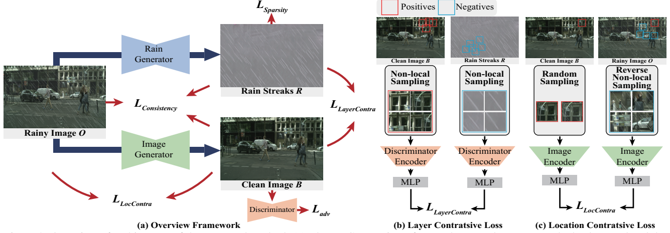
Figure 3. Overview of architecture of the proposed method. (a) The NLCL consists of two sub-networks to extract the background and the rain layers respectively with two additional contrastive constraints. (b) The layer contrastive between the clean image and rain streaks with the non-local sampling for both positives and negatives. (c) The location contrastive between the clean image and rainy image with the reverse non-local sampling for negatives.
