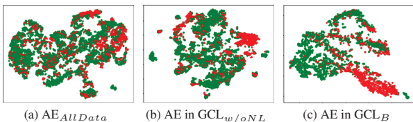
Figure 6. tSNE [53] visualizations of the reconstructions. Using GCL_B , most of the anomalous samples (red) get clustered separately from the normal samples (green), which is the underlying desideratum of providing pseudo reconstruction targets.
