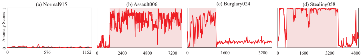
Figure 8. Anomaly scores by GCL_{PT} are low in normal regions and high in abnormal regions on four different UCFC videos.
