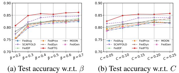
Figure 5. (a) Test accuracy w.r.t. data heterogeneity. (b) Test accuracy w.r.t. fraction C of active clients in each round ( \beta = 0.3 ). All experiments are conducted on CIFAR100.
