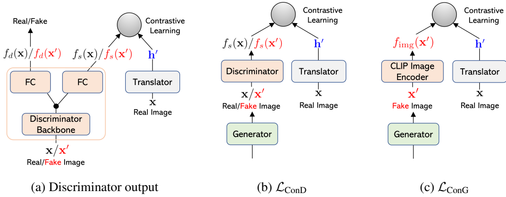
(a) Discriminator output (b) \mathcal{L}_{\text{ConD}} (c) \mathcal{L}_{\text{ConG}} Figure 4. Illustration of discriminator outputs and training objectives for the language-free setting.
