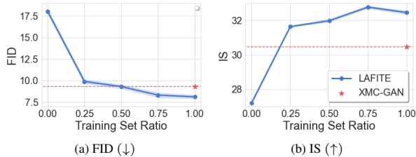
Figure 7. Comparison of LAFITE and prior art XMC-GAN. X-axis is the percentage of image-text pairs in the full MS-COCO dataset. XMC-GAN has over 166 millions trainable parameters, while our LAFITE only has 75 millions trainable parameters.
