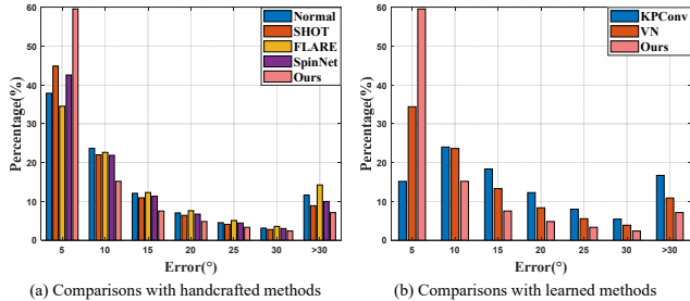
Figure 3. Histogram of the orientation repeatability on the 3DMatch dataset, where the errors denote the deviation angles of estimated orientations between the ground-truth point pairs.
