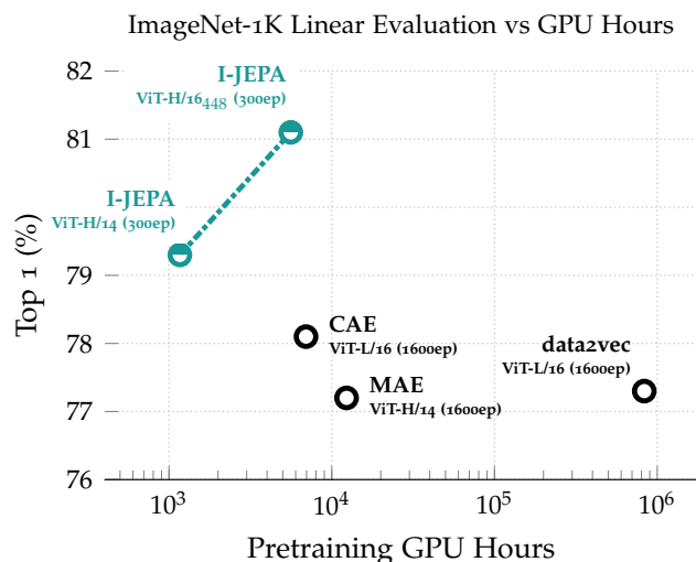
Figure 1. ImageNet Linear Evaluation. The I-JEPA method learns semantic image representations without using any view data augmentations during pretraining. By predicting in representation space, I-JEPA produces semantic representations while using less compute than previous methods.
