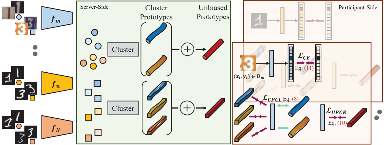
Figure 2. Architecture illustration of Federated Prototypes Learning (FPL). Participants upload local prototypes to server. Based on these prototypes, we introduce cluster prototypes ( ) to construct Cluster Prototypes Contrastive Learning (CPCL in Sec. 3.3.1), bringing diverse domain information. Besides, we acquire unbiased prototypes ( ) and propose Unbiased Prototypes Consistent Regularization (UPCR in Sec. 3.3.2) to provide a stable consistency signal. Best viewed in color. Zoom in for details.
