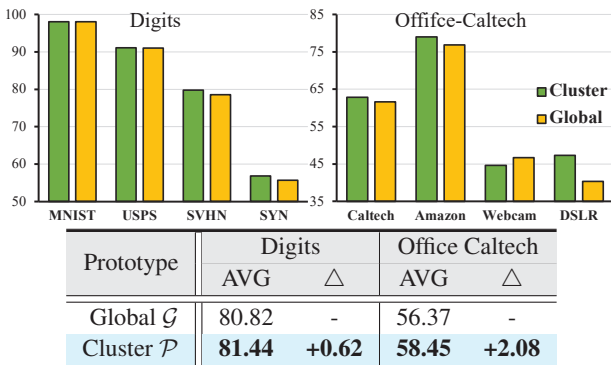
Figure 5. Comparison of cluster ( \mathcal{P} in Eq. (5)) and global prototypes ( \mathcal{G} in Eq. (3)) for CPCL (Sec. 3.3.1) on each domain (Top Row) and overall performance (Bottom Row) in Digits and Office Caltech tasks with \tau = 0.02 . See details in Sec. 4.2.1.
