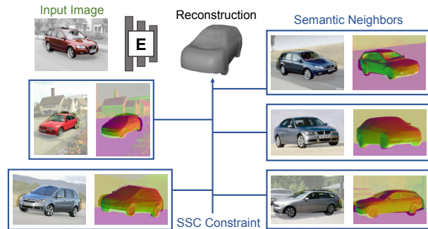
Figure 3. Semantic-based Shape Consistency (SSC) Constraint. We find the semantic neighbors of the input image across the training set and use these neighbors to regularize the shape learning.
