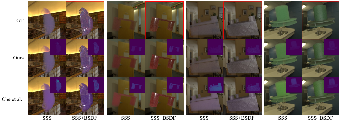
Figure 4. Visual comparison with Che et al. [11]. We use two visualizations which are “SSS” and “SSS+BSDF” to show the parameter estimation results. “SSS” is rendered by the GT illumination, shape, and predicted SSS. “SSS+BSDF” is rendered by the GT illumination, shape, BxDF, and predicted SSS. Images in red rectangles are input images. Error maps are in the upper right corner.
