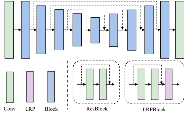
Figure 3. Network architecture for scene segmentation. We use the sparse convolutional U-Net [29] as our baseline, consisting of four stages. For the baseline, we use ResBlock as the basic block to extract features, and we replace the ResBlock with LRPBlock to build LRPNet.
