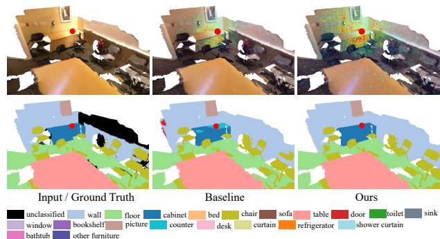
Figure 1. Qualitative results of Effective Receptive Field (ERF) [45]. Left: the input and ground truth. Middle: the ERF and results of baseline described in section 3.3. Right: the ERF and results of LRPNet (ours). The stained areas around the positions of interest (red dots) represent the range of receptive fields, with green to red representing the increasing strength of response. Our method correctly segments the cabinet from the wall with the proposed effective receptive field.
