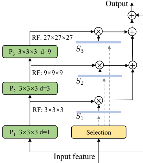
Figure 2. Long Range Pooling Module. Dilation max pooling is used to enlarge the receptive field and also outputs features of the different receptive field. P_1, P_2, P_3 : max pooling with kernel size 3 \times 3 \times 3 and dilation 1, 3, 9. RF : the receptive field. Selection : a linear module producing the selection weight for each voxel.
