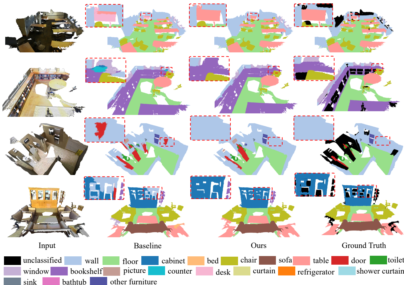
Figure 4. Various ScanNet v2 validation set segmentation results. Red dotted boxes highlight differences between our results and the baseline results.
