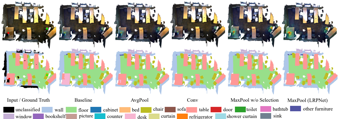
Figure 5. Visualization of Effective Receptive Field (ERF). Red Dot and Green Pentagon : two different positions of interest (marked only in the input). First Row : the ERFs of different methods. Second Row : the ground truth and predictions. From Left to Right : input, baseline, average pooling, convolution, max pooling without selection, max pooling (LRPNet).
