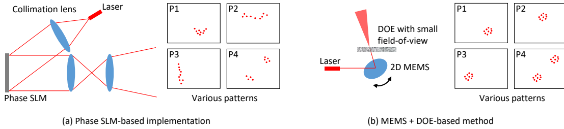
Figure 4. Hardware implementations. (a) Our first implementation is based on a phase-only SLM, which can redistribute light to arbitrarily-shaped, even disjointed ROIs. (b) Our second implementation is based on a DOE pattern generator with a 2D MEMS mirror. It has less flexibility and can only concentrate on one fixed-shape ROI at a time, but it benefits from low cost, simple optics and small form factor which makes it potentially easier to be miniaturized.
