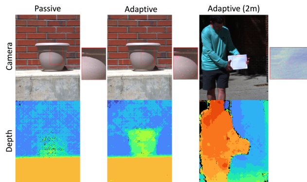
Figure 8. Outdoor active depth sensing under 50 kilolux direct sunlight with Phase SLM. Our sensor works outdoors under direct sunlight. We show results up to 2 meters but believe this range could be extended with further SLM optical engineering. Zoom in to see the red dots in the camera images.
