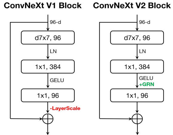
Figure 5. ConvNeXt Block Designs. In ConvNeXt V2, we add the GRN layer after the dimension-expansion MLP layer and drop LayerScale [41] as it becomes redundant.
