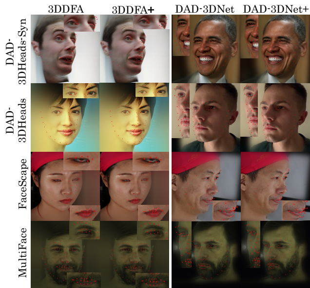
Figure 6. The visual comparisons between baseline methods and the refined methods on four testing sets. The left column and upper row list the dataset and method names, respectively. '+' denotes the model that has been refined by our 3D-aware training.
