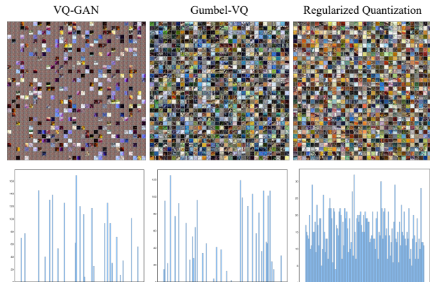
Figure 1. Visualization of codebook (first row) and illustration of codebook utilization (second row) on ADE20K dataset [42]. VQ-GAN [8] severely suffers from codebook collapse as most codebook embeddings are invalid values. Gumbel-VQ [2] learns valid values for all codebook embeddings, while only a small number of embeddings are actually used for quantization as illustrated in codebook utilization. As a comparison, the proposed regularized quantization prevents codebook collapse and achieves full codebook utilization. The codebook visualization method is provided in the supplementary file.
