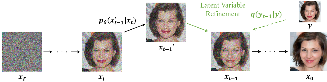
Figure 2: Graphical model of Iterative Latent Variable Refinement. From state x_t , we first sample unconditional proposal x_{t-1} according to Eq. 5. Then, we match latent variable with encoded condition y_{t-1} according to Eq. 8.
