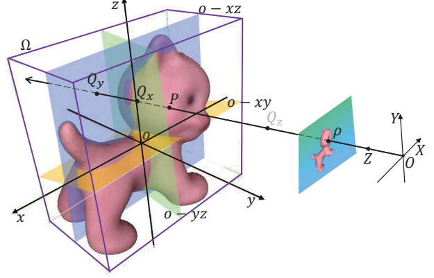
Figure 3. Demonstration of self-occlusion. The ray OP from camera center O towards the visible point P intersects the object coordinate planes o - yz , o - xz , o - xy at 3 points Q_x , Q_y and Q_z . We only consider the points inside the pre-defined region \Omega for training stability, thus Q_z would be removed in this example.
