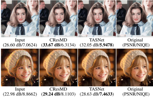
Figure 5: Non-blind qualitative image quality comparison. TASNet produces sharper images with better NIQE scores than CResMD.
