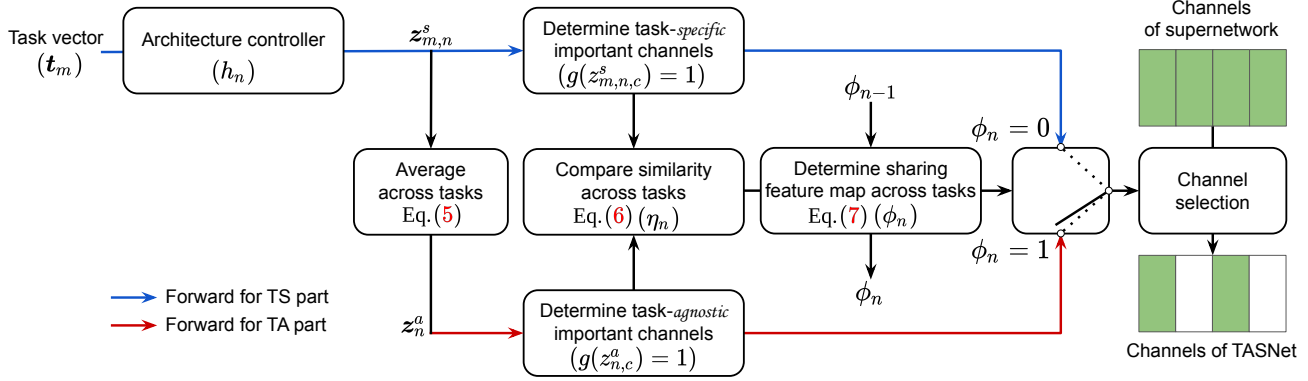
Figure 3: The neural architecture search process for each layer of TASNet. Our algorithm automatically determines the number of shared layers and channels in each feature map from the supernetwork. Task-specific (TS) part ( \phi_n = 0 ) adaptively selects channels based on the given task (blue arrow). By contrast, task-agnostic (TA) part ( \phi_n = 1 ) selects fixed channels across tasks (red arrow). A feature map is determined to be shared if the channel importance is similar among tasks and the previous feature map is shared. All processes are differentiable via a straight-through estimator ( g ). During the inference, \phi , z^a , and thus task-agnostic (TA) part are fixed.
