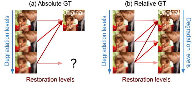
Figure 4: Absolute ground truth vs. relative ground truth. (a) Mapping from all degraded versions to its original image. (b) Mapping from degraded versions to relatively higher-quality images.
