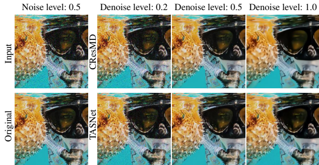
Figure 7: Blind setting (over-smoothing) . When denoise levels are higher than the actual noise levels of input images, CResMD over-smoothes images whereas TASNet noticeably removes noise.
