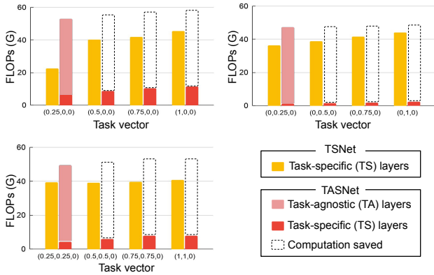
Figure 11: Computation cost comparisons across restoration levels. The higher restoration levels demand more computation costs for TS layers. TASNet is efficient for multiple inferences, as a result of reusing the feature map of TA layers across tasks. Each graph presents computation costs of removing blur (upper left), noise (upper right), and joint degradation of blur and noise (lower left). A task vector (\cdot, \cdot, \cdot) denotes the levels of (Deblur, Denoise, Dejpeg).
