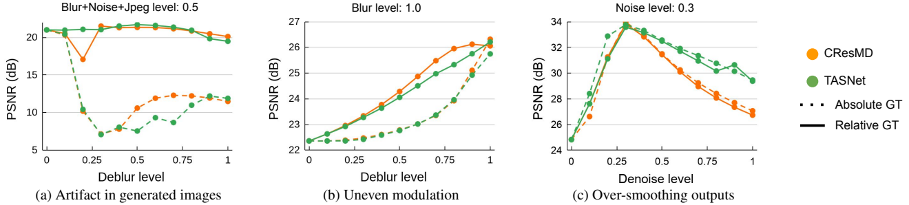
Figure 10: Ablation study for three image modulation problems in the blind setting. Models trained by relative GT reduce (a) network artifact generation when deblurring images corrupted by a mixture of degradation types and (b) uneven image modulation across deblurring levels. Further, task-agnostic feature maps from TASNet prevent (c) over-smoothing outputs.
