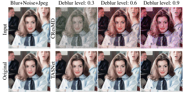
Figure 6: Blind setting (artifact) . CResMD often produces significant artifacts when deblurring images that are corrupted with noise or compression artifacts. By contrast, TASNet successfully reduces the blur in input images.
