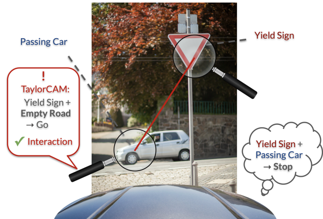
Figure 1: An automated driver decides whether to “stop” or “go.” Here, the decision cannot be explained by individual factors alone, but by the interaction between the yield sign and the passing car. Taylor-CAM identifies interactions by considering how changing one object affects the significance of another, such as how changing a passing car into an empty road would change the meaning of the yield sign from “stop” to “go.”
