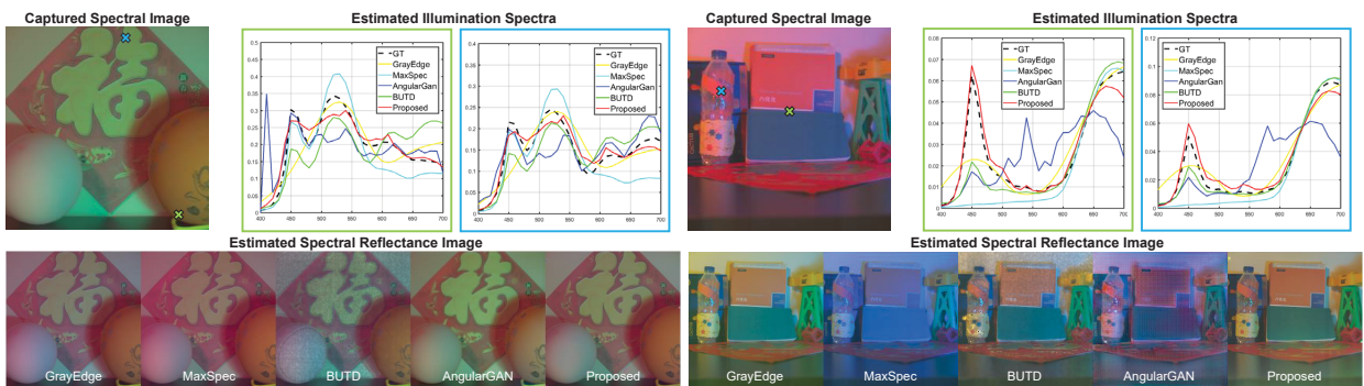
Figure 7. The comparisons of the estimated illumination spectra and reflectance images. Both scenes were illuminated by two full-spectrum lamps with filters. We show the estimated spectra of the five illumination estimation methods at the positions of two crosses in each scene. The reflectance images are rendered to RGB images for visualization.
