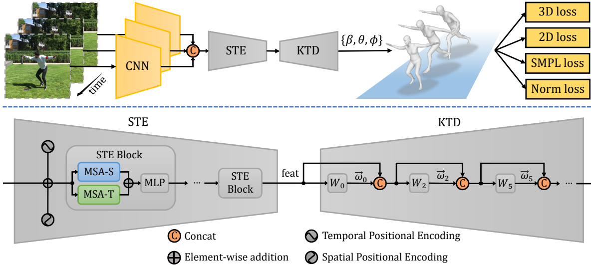
Figure 2: Overview of the proposed method MAED. The upper part shows the pipeline of the model and the lower part presents the structures of our proposed Spatial-Temporal Encoder and Kinematic Topology Decoder.
