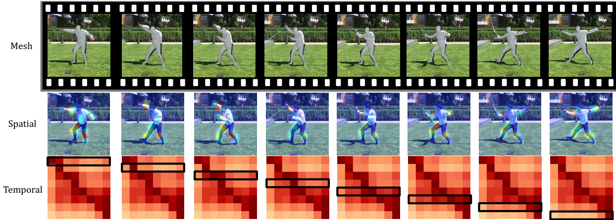
(a) Extreme Pose. Spatial attention is mainly concentrated on human joints, while temporal attention is mainly concentrated near the anchor frame.
