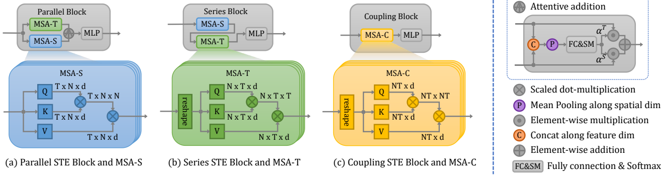
Figure 3: STE block variants and MSA variants.
