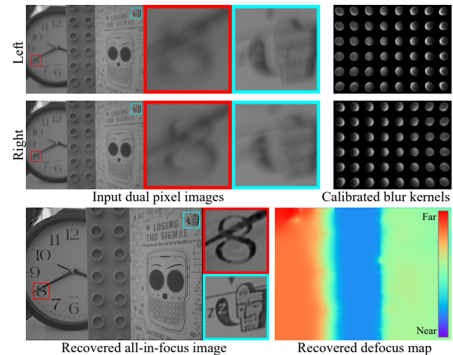
Figure 1: Given left and right dual-pixel (DP) images and corresponding spatially-varying blur kernels, our method jointly estimates an all-in-focus image and defocus map.
