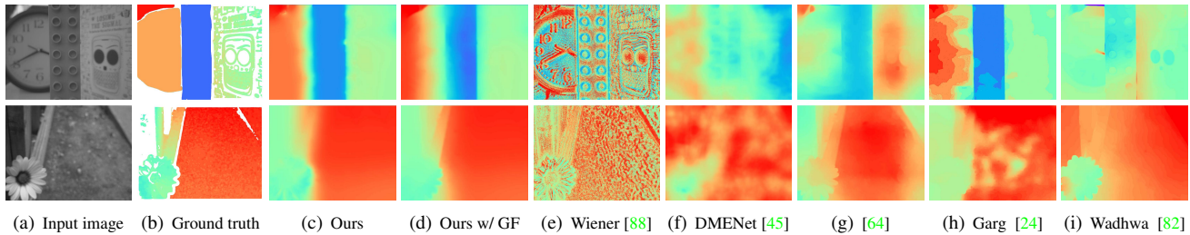
Figure 7: Qualitative comparisons of defocus map estimation methods. Input images (a) shown as the average of two DP views, ground truth defocus maps (b) from focus stacks with zero confidence pixels in white, our defocus maps (c), and our defocus maps with guided filtering (d), and defocus maps from other methods (f)-(i). Overall, our method produces results that are closest to the ground truth, and correctly handles textureless regions as well.
