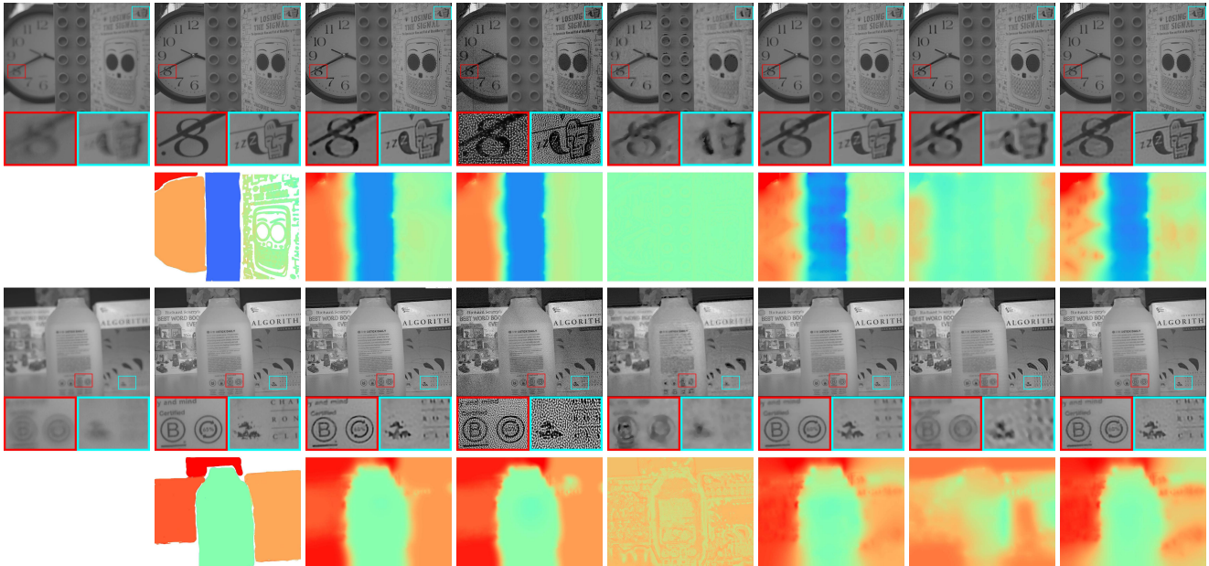
(a) Input image (b) Ground truth (c) Ours full (d) No \mathcal{L}_{intensity} (e) No \mathcal{L}_{alpha} (f) No \mathcal{L}_{entropy} (g) No \mathcal{L}_{aux} (h) No \mathcal{B}
