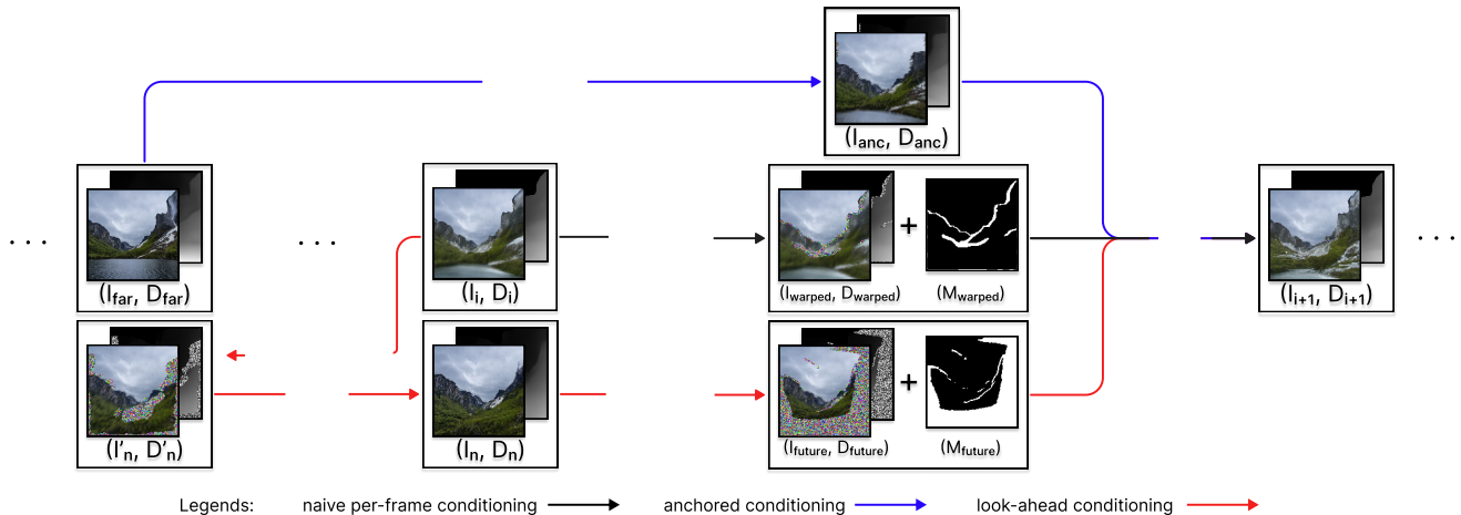
Figure 2: Overview of our pipeline. We train an image-conditional diffusion model to perform image-to-image refinement and inpainting given a corrupted image and its missing region mask. At inference, we perform stochastic conditioning on three conditionings: naive forward warping from the previous frame (black arrow), anchored conditioning by warping a further frame (blue arrow), and lookahead conditioning by warping a virtual future frame (red arrow). We repeat this render-refine-repeat pipeline to get sequences extrapolating a given image.
