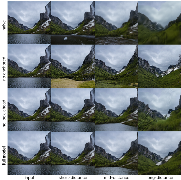
Figure 7: Ablation study , where we disabled our key building blocks. We observe clear artifacts (naive, no lookahead) or inconsistency (no anchored) in all ablations.
