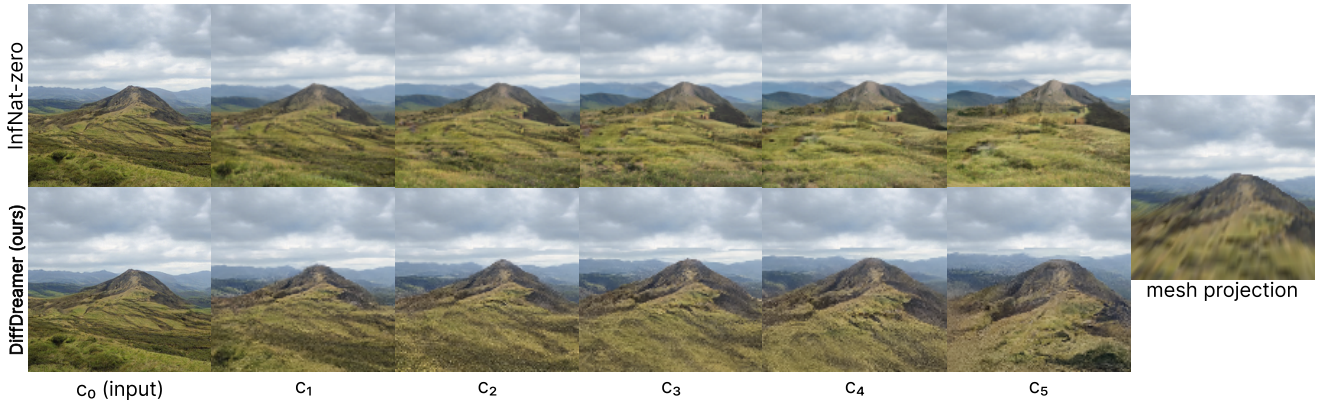
Figure 5: Comparison of 3D consistency achieved by our DiffDreamer and InfNat-0 [40], where we ask the camera to fly towards the top of the hill and show the intermediate renderings at camera positions c_0 to c_5 .
